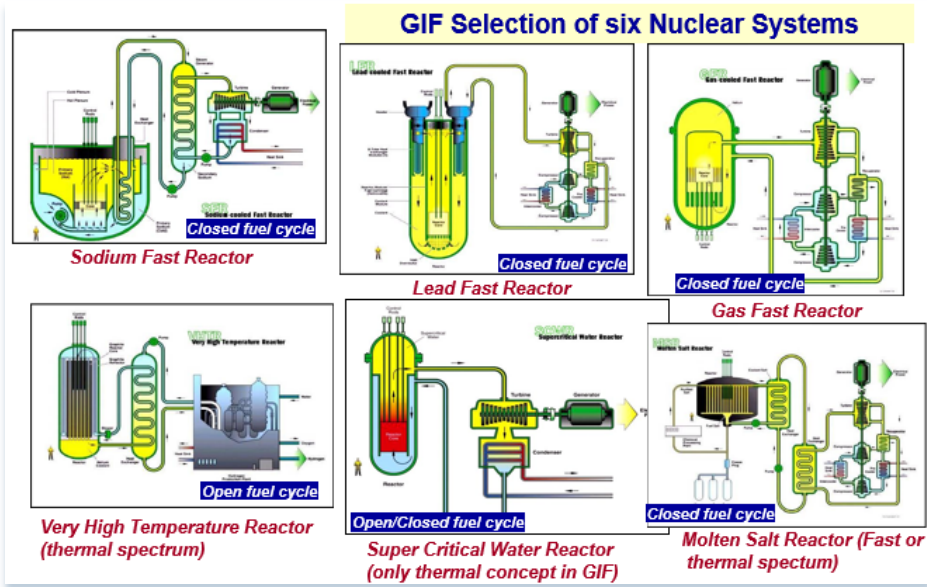
Figure 2: The six GIF systems, four of which use a closed fuel cycle and a fast spectrum
