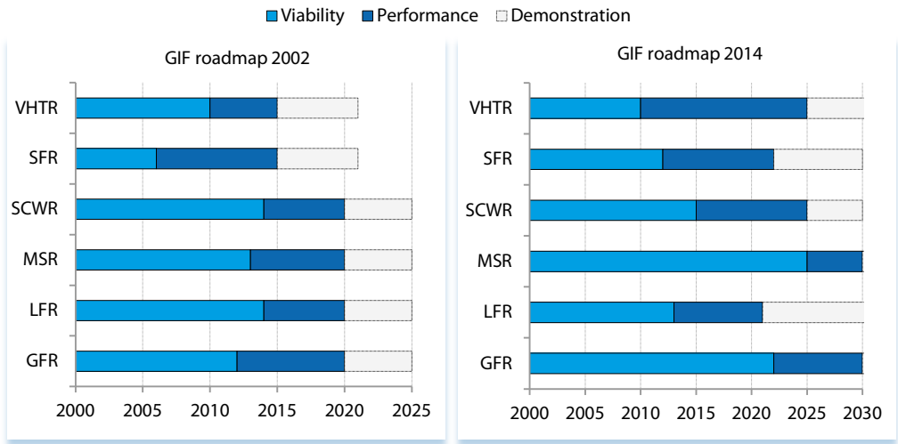
Figure 3: TRL level for the six GIF systems (2014 update of the Technology Roadmap)
